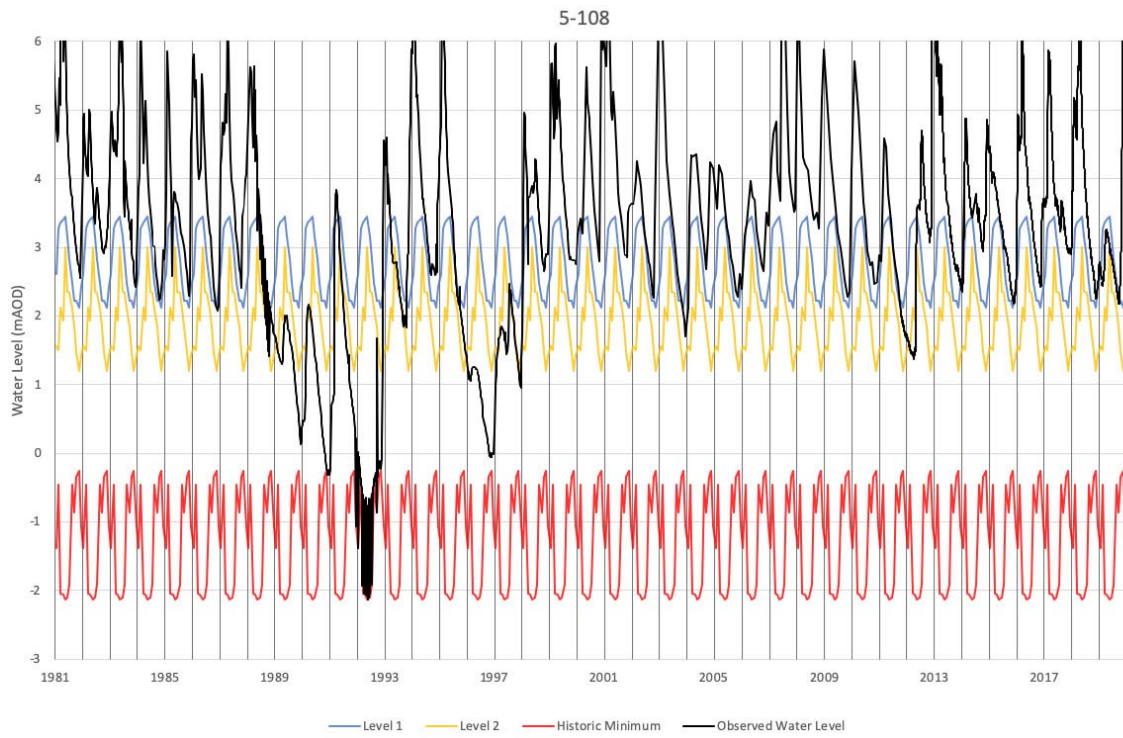
Figure 3.6: Drought management curves used for Goxhill 2
