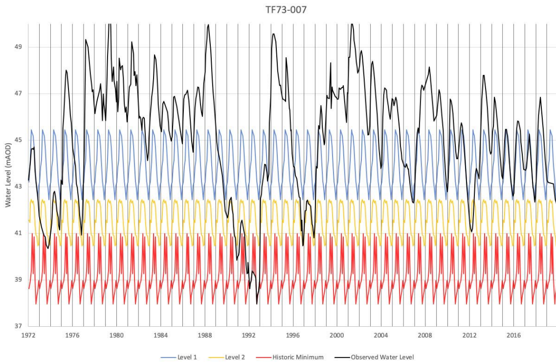
Figure 3.17: Drought management curves used for Fring Osier Carr and Sedgeford
