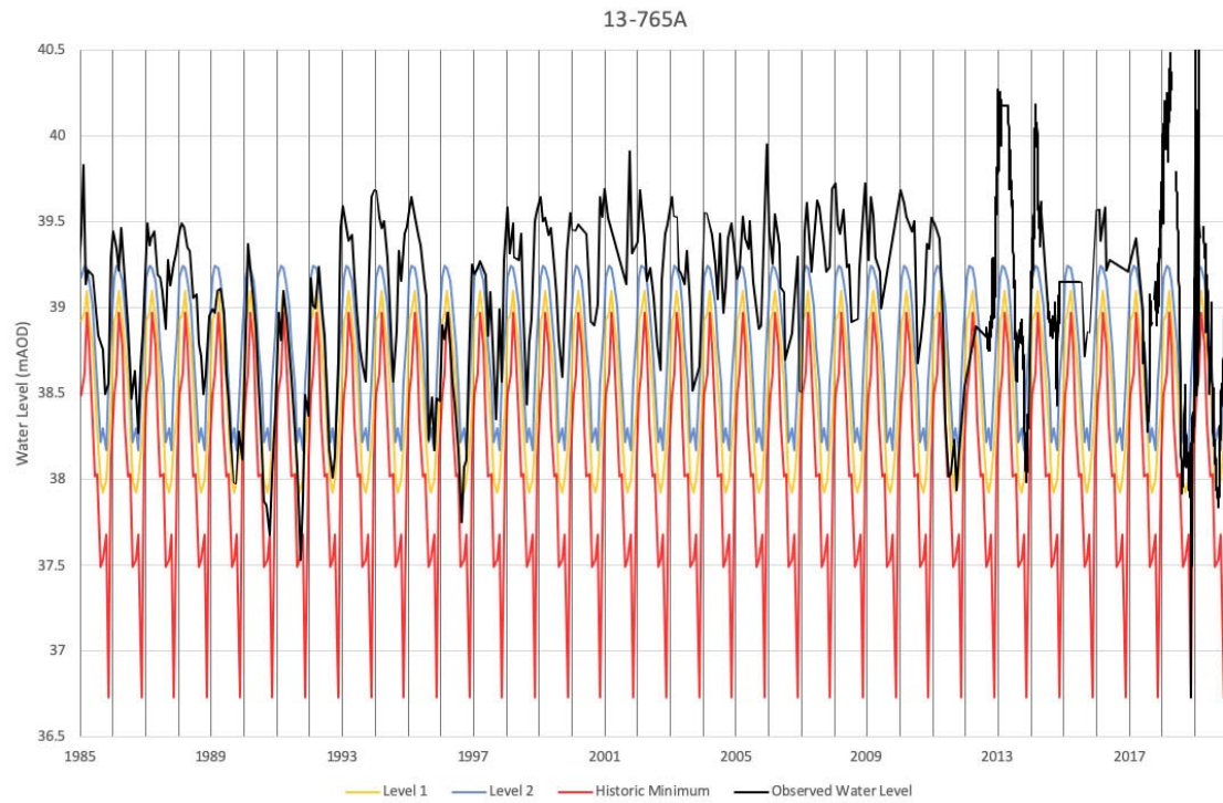
Figure 3.8: Drought management curves used for Metton
