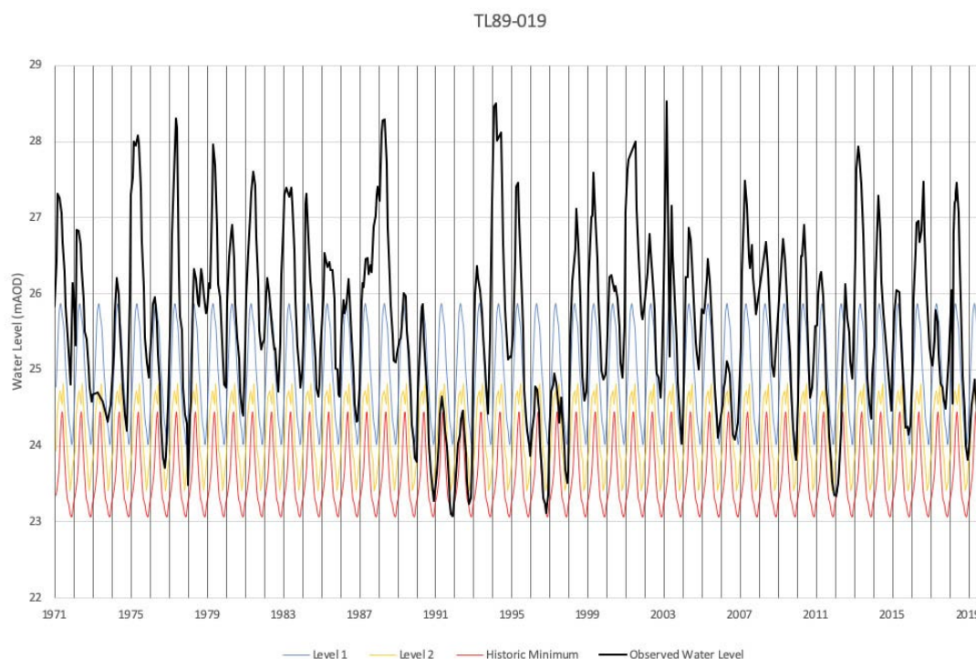
Figure 3.2: An example of the new curves plotted against the actual observed water level for the historic record of the Environment Agency observation borehole TL89/019 in the West Norfolk Wissey Chalk
