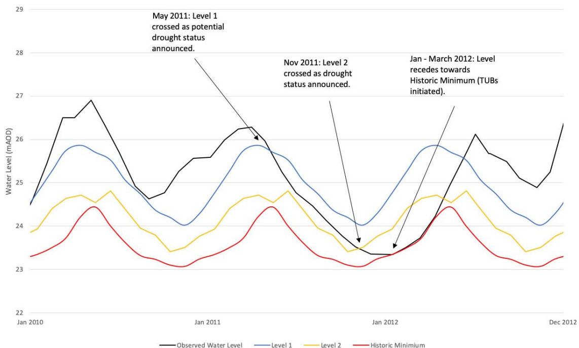
Figure 3.3: Worked example of the drought management curves for the 2011/12 drought
